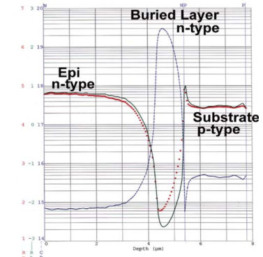
n-doped Epi on Sb Buried Layer
