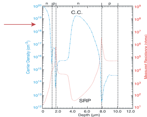
Carrier Density Analysis
