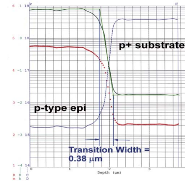
p on p+ epi transition width
