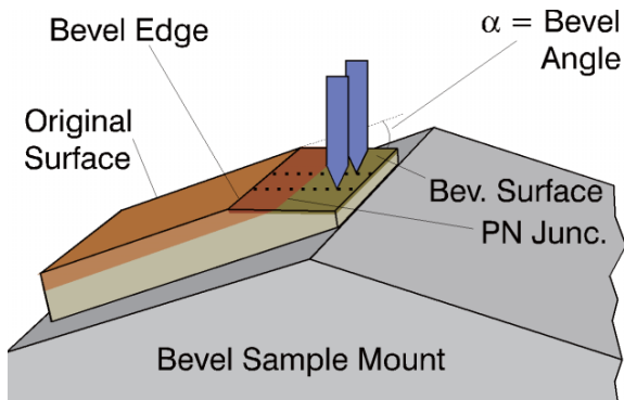
Standard SRP setup
